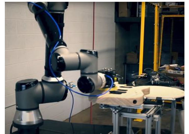
Assembly
